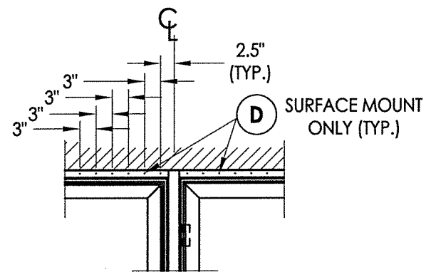
MULLION ANCHORING DETAIL Vertical and horizontal orientation (See sheet 10 for remaining anchoring for horizontal orientation)
