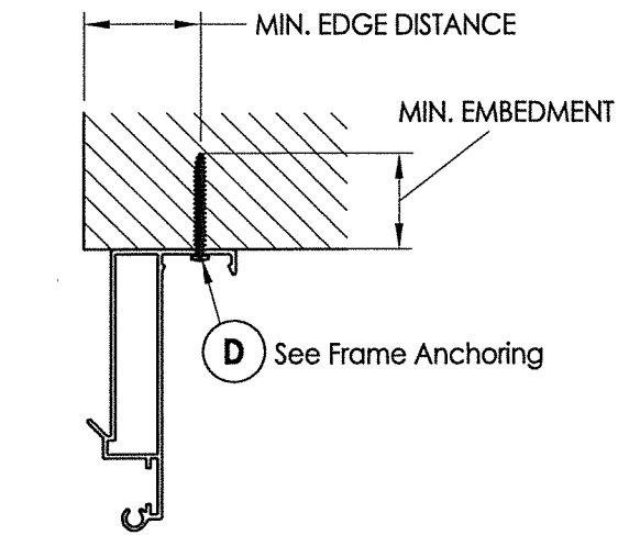
SURFACE MOUNT ANCHORING
