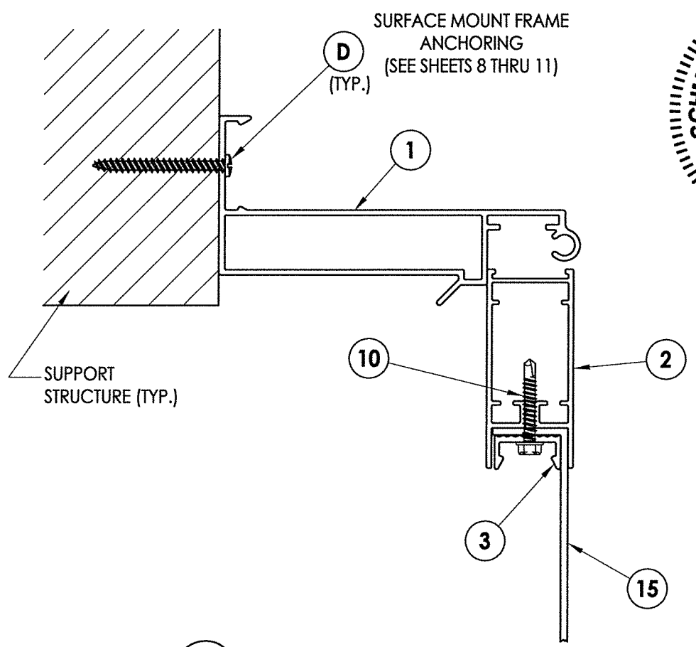
2 6 VERTICAL CROSS SECTION
