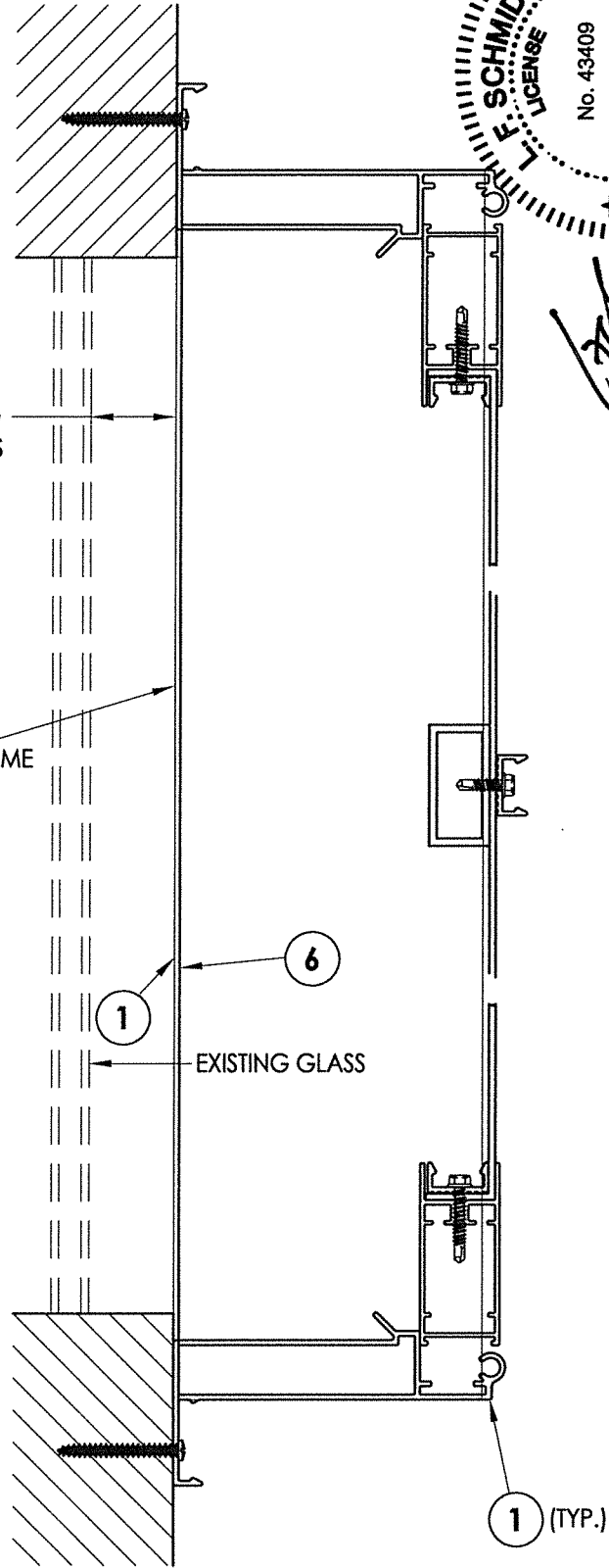
MULTIPLE MULLED PANELS GLASS SEPARATION Vertical orientation only
