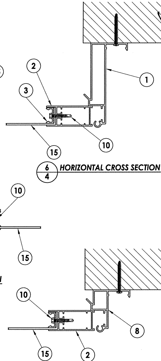
8 4 HORIZONTAL CROSS SECTION
